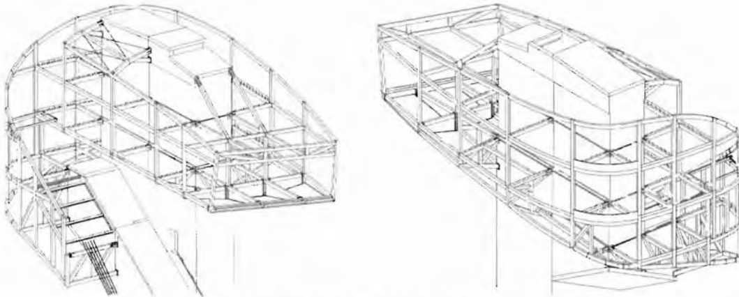
Fig. 14 Tower top - sketch of the steelwork construction
