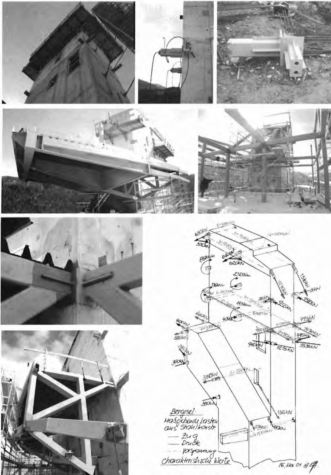
Fig. 16 Docking solution between concrete tower and steel cage with prestressed bearing brackets
