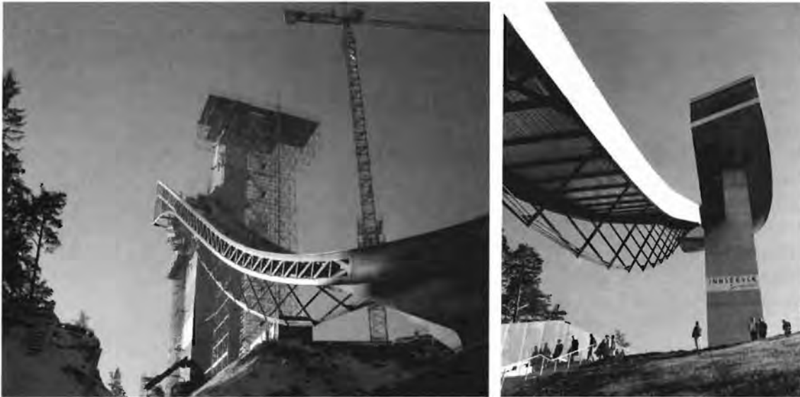
Fig. 7 Tower and column-free approach ramp
