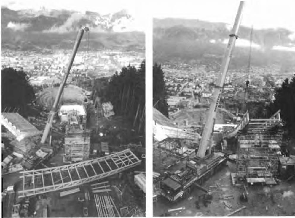
Fig. 10 Lifting of the first part of the approach ramp
